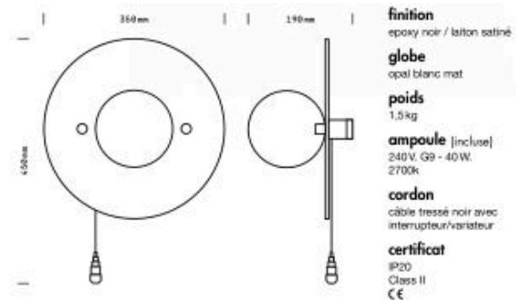
Dimensions fixation murale
